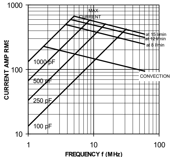
Fig. 8: Typical current vs. frequency and capacitance Example: CVLA-1000BW/50-ZJP-R
