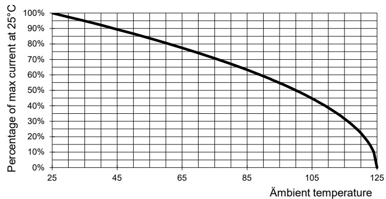
Fig.5: Derating RF current in percent of maximum permissible current at 25° C ambient temperature
