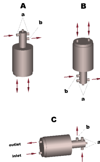
Fig. 9: Vacuum capacitors with water flow up to 15 l/minute
