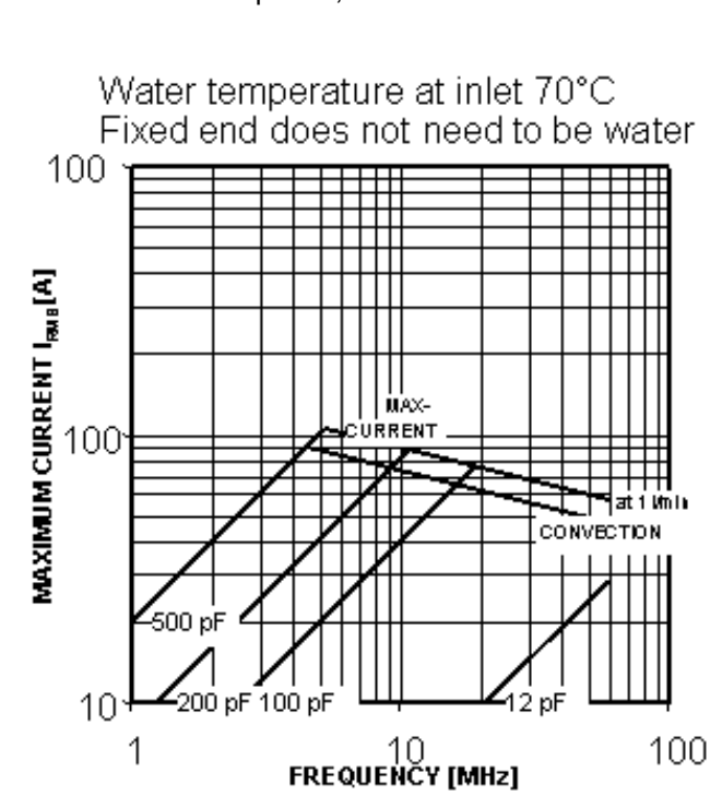
Fig. 13: Current curve CVMI-500AW/15-AAC-M
