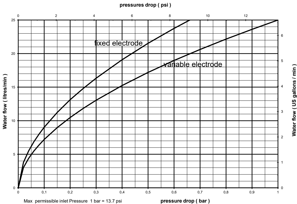
Fig. 12: Pressure drop across capacitor vs. water flow (typical)
