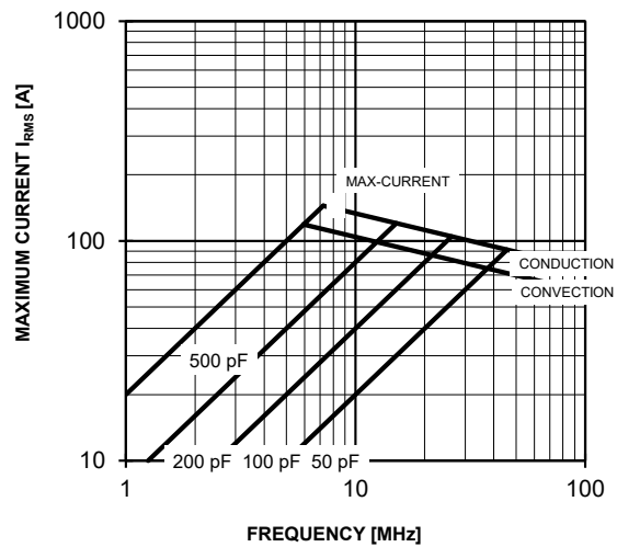
Fig 6: Typical current vs. frequency and capacitance Example: CVPO-500BC/7.5-BECA
