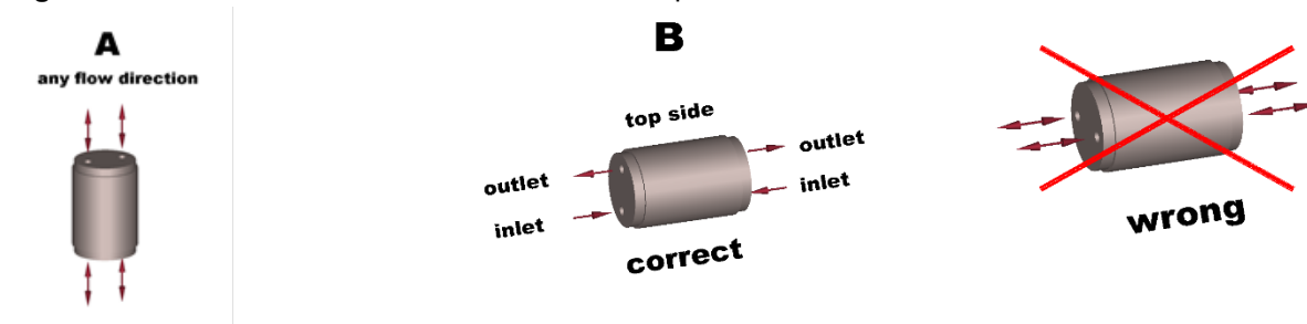
Fig. 11: Water connections for water-cooled fixed capacitors
