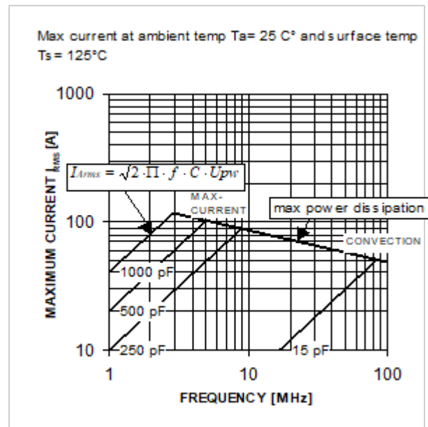
Fig. 2: Typical current vs. frequency and capacitance Example: CVBA-500BC/8-BEA-L
