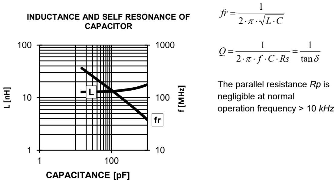
Fig. 4: Typical inductance and self-resonance of variable capacitor vs. capacitance Example: CVBA-500BC/5-BEA-L
