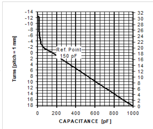
Fig 3: Typical turns vs. capacity Example: CVBA-500BC/5-BEA-L
