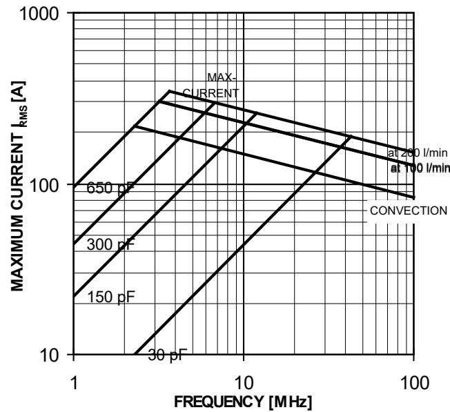
Fig 6: Typical current vs. Frequency and capacitance Example: CVMA-650AA/55-ABB
