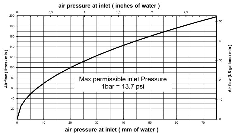
Fig. 7: Air flow vs. air pressure (typical)
